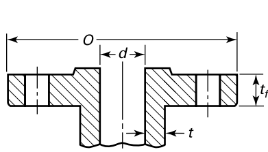
Flanged Fitting
