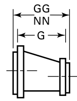
Eccentric Reducer
