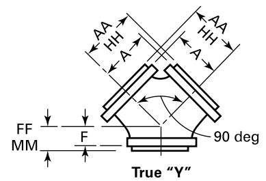
True "Y"
