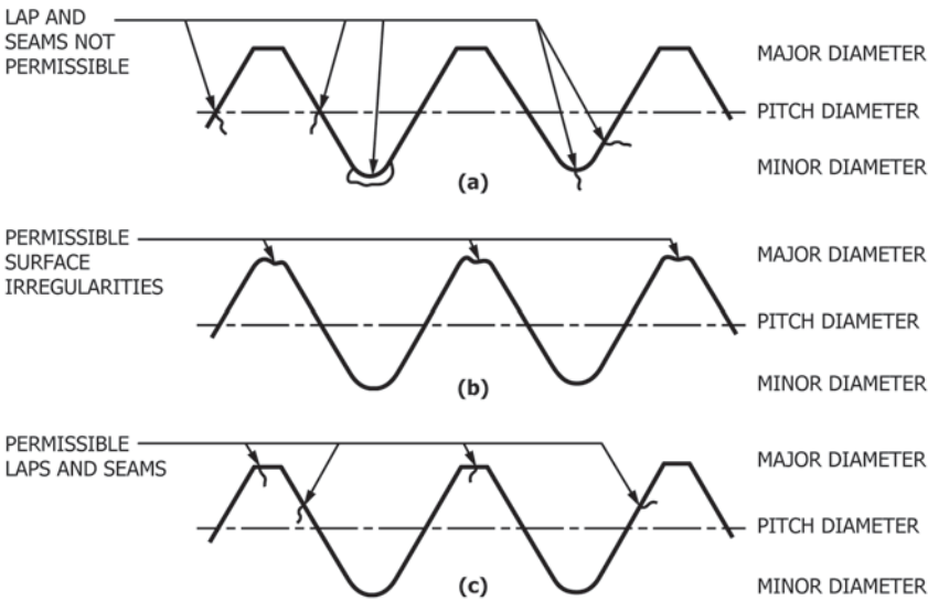
FIG. 3 Thread Discontinuities
